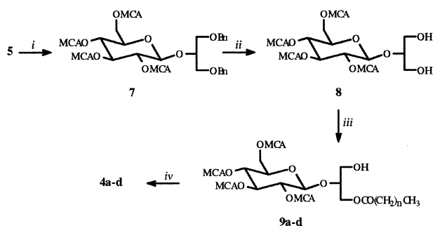
Scheme 2. Reagents: (i) (\text{ClCH}_2\text{CO})_2\text{O} , \text{CH}_2\text{Cl}_2/\text{Py} , 0°C; (ii) \text{H}_2 , Pd/C; (iii) LCA, \text{CF}_3\text{CH}_2\text{OCO}(\text{CH}_2)_n\text{CH}_3 , THF; (iv) \text{NH}_2\text{NH}_2\cdot\text{AcOH} , \text{AcOEt}/\text{MeOH} ; MCA = \text{COCH}_2\text{Cl} .
