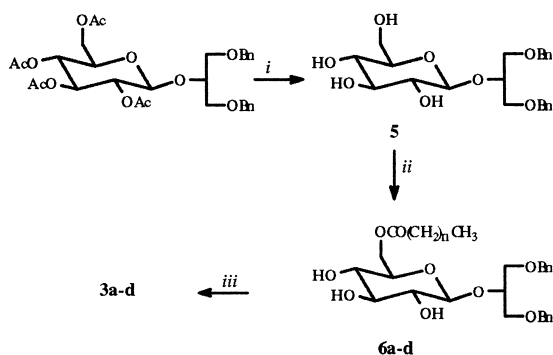
Scheme 1. Reagents: (i) MeOH, MeONa; (ii) LPS, \text{CF}_3\text{CH}_2\text{OCO}(\text{CH}_2)_n\text{CH}_3 , THF; (iii) \text{H}_2 , Pd/C.
